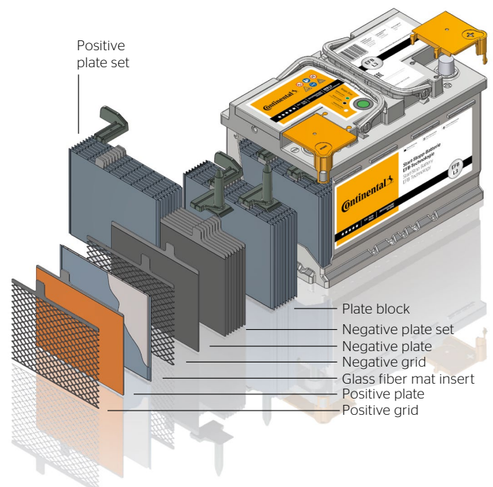
EFB technology: Battery construction
